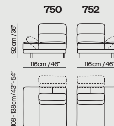
Seat with adjustable arm and backrests
